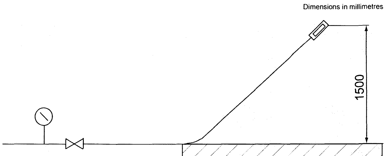
Figure E.1 — Arrangement for impact test
